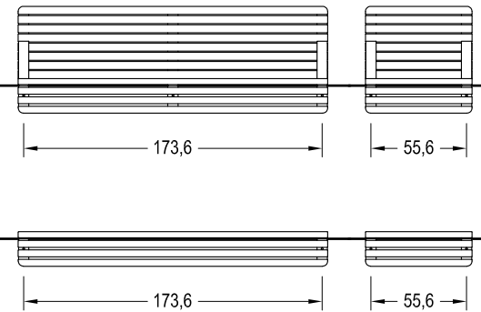
C. UNIVERSE banca / backless bench
