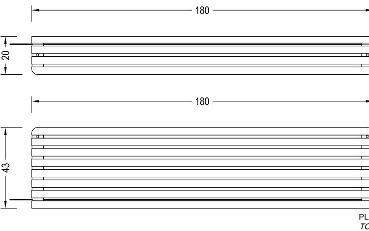
C. UNIVERSE banca / backless bench
