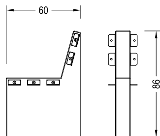
Soporte Banco Derecho 95 kg Ref. ALPINE-BCO-DRCH
