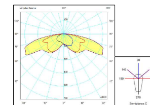
LED 4C
