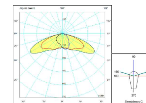
Microreflector 90W-140W
