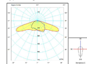
LED 3C
