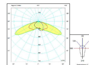
Microreflector 45W-60W
