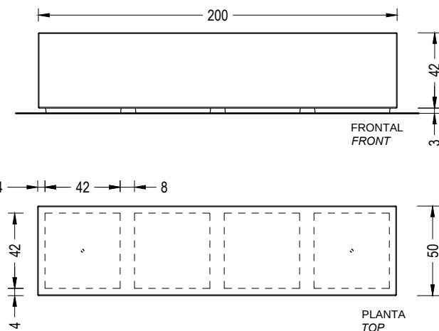
BOX 200
