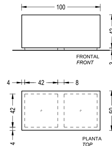
BOX 100
