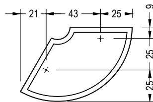
BOX RADIUS 120°
