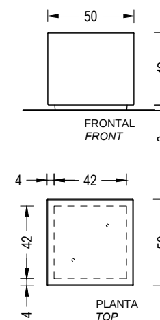
BOX 50
