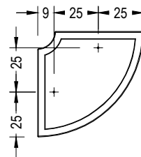
BOX RADIUS 90
