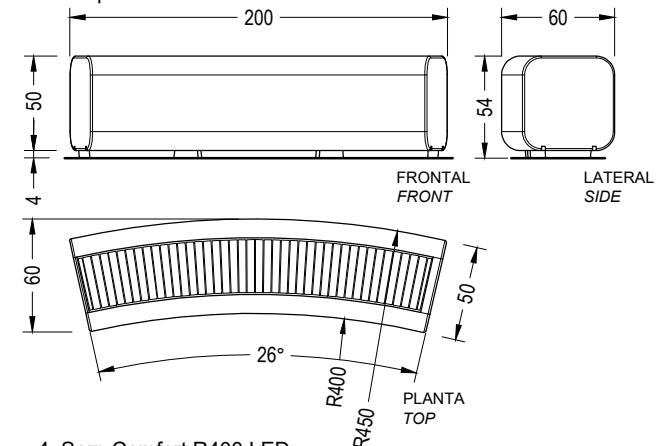
4. Serp Comfort R400 LED
