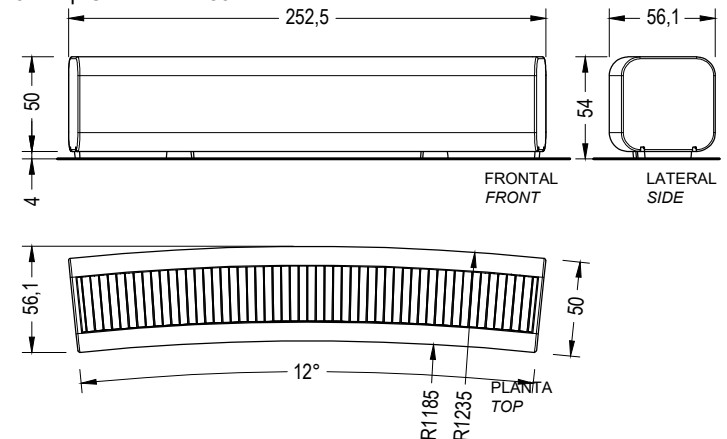
4. Serp Comfort R1185 LED
