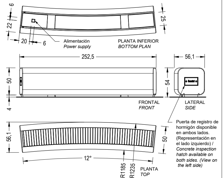
4. Serp Comfort R1185 LED
