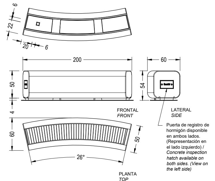
4. Serp Comfort R400 LED
